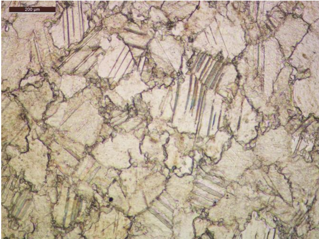
Figure 1. The photograph shows the microstructure of the grains as well as grain size. Note smaller grains (~0,05 mm) along grain boundaries. Note also scale bar at the top left of the photo.
